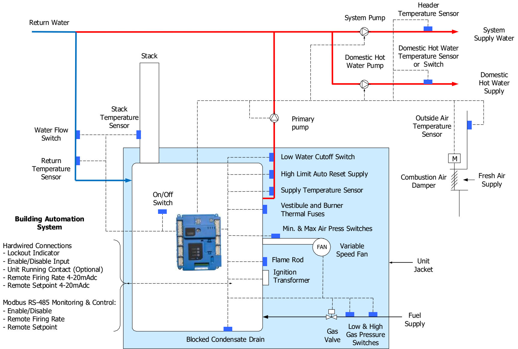
Figure 3: Unit Control
